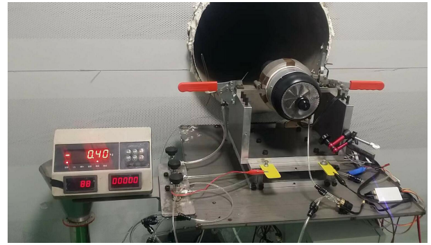
Test bench(option)
